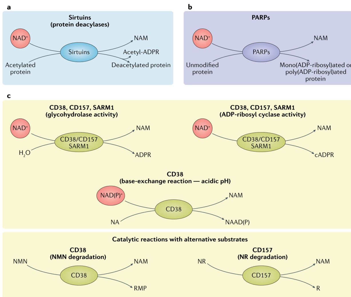
Fig. 2 |. Three main classes of \text{NAD}^+ -consuming enzymes.
